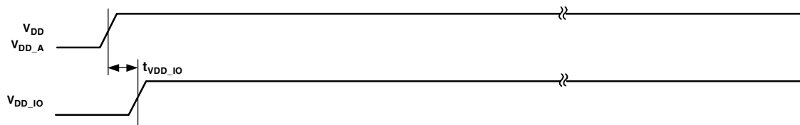
Figure 12. Power-Up Sequencing Timing
