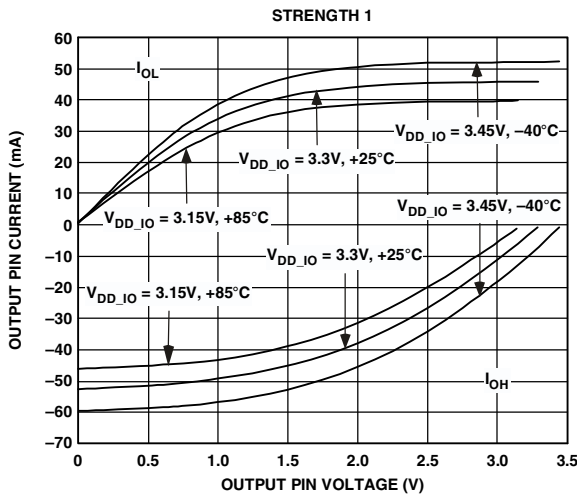
Figure 21. Typical Drive Currents at Strength 1
