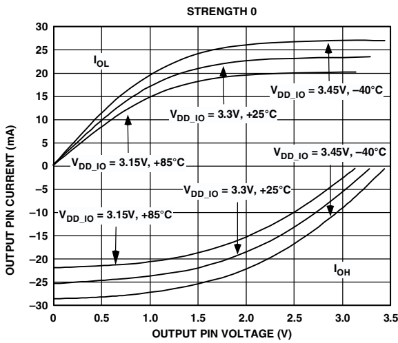
Figure 20. Typical Drive Currents at Strength 0
