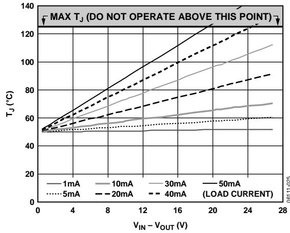
Figure 25. 300 mm 2 of PCB Copper, T A = 50°C
